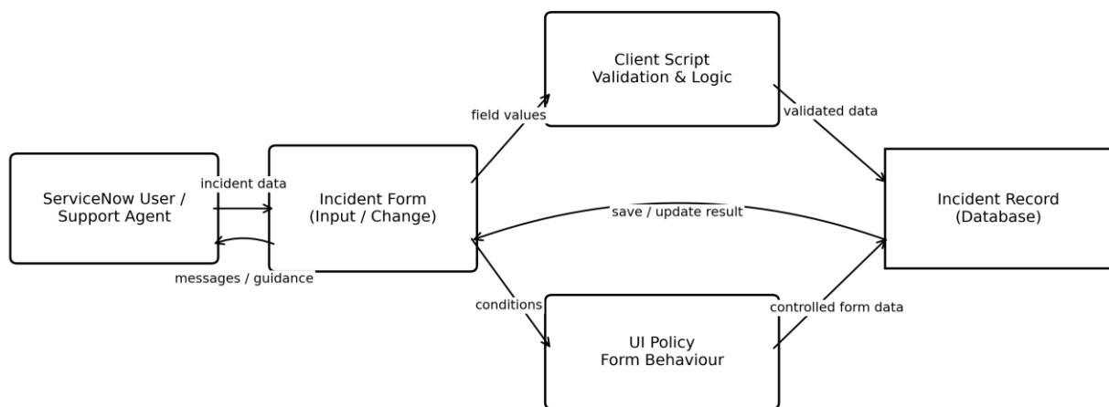
ServiceNow Incident - Client Script & UI Policy Data Flow
